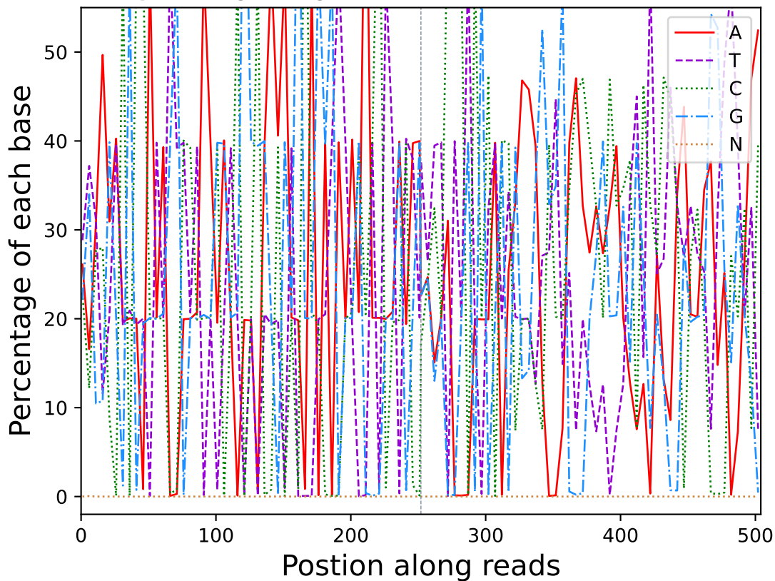
Base percentage along reads (R10506)
